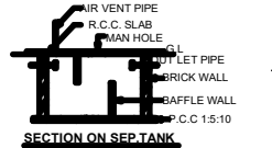
SECTION ON SEPT. TANK
