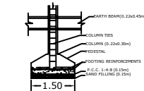
FOUNDATION DETAILS
