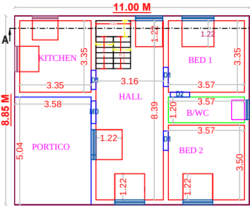
PLAN - GROUND FLOOR (PROPOSED)
