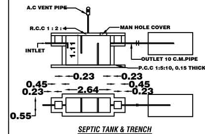
SEPTIC TANK & TRENCH
