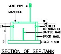
SECTION OF SEP.TANK
