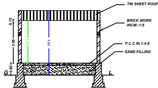
SECTION "AR"
