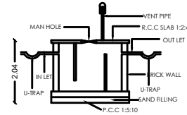
SECTION E.F. SEPTIC TANK DETAIL
