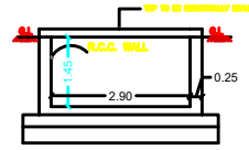
RWH SECTION
