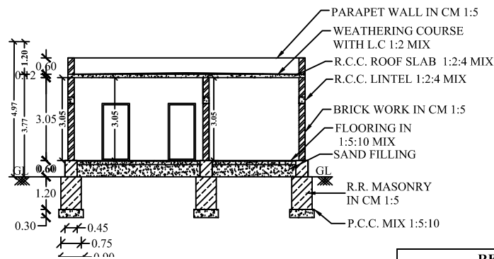
SECTION OF "AB"
