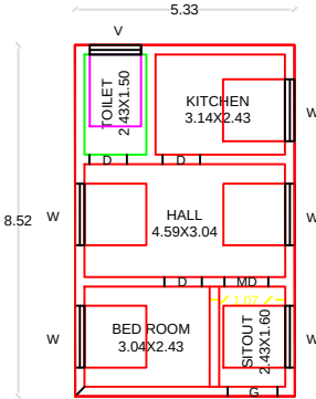
PROPOSED GF PLAN
