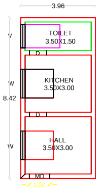
PRO GF PLAN
