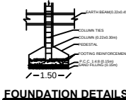
FOUNDATION DETAILS
