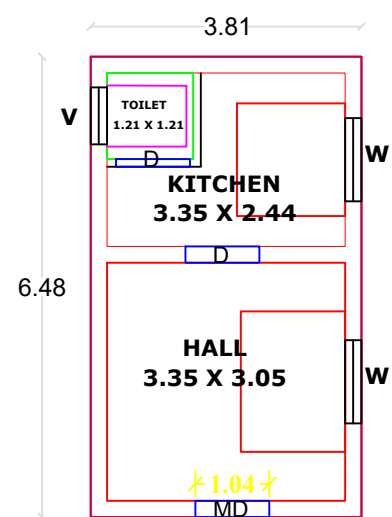
PLAN
