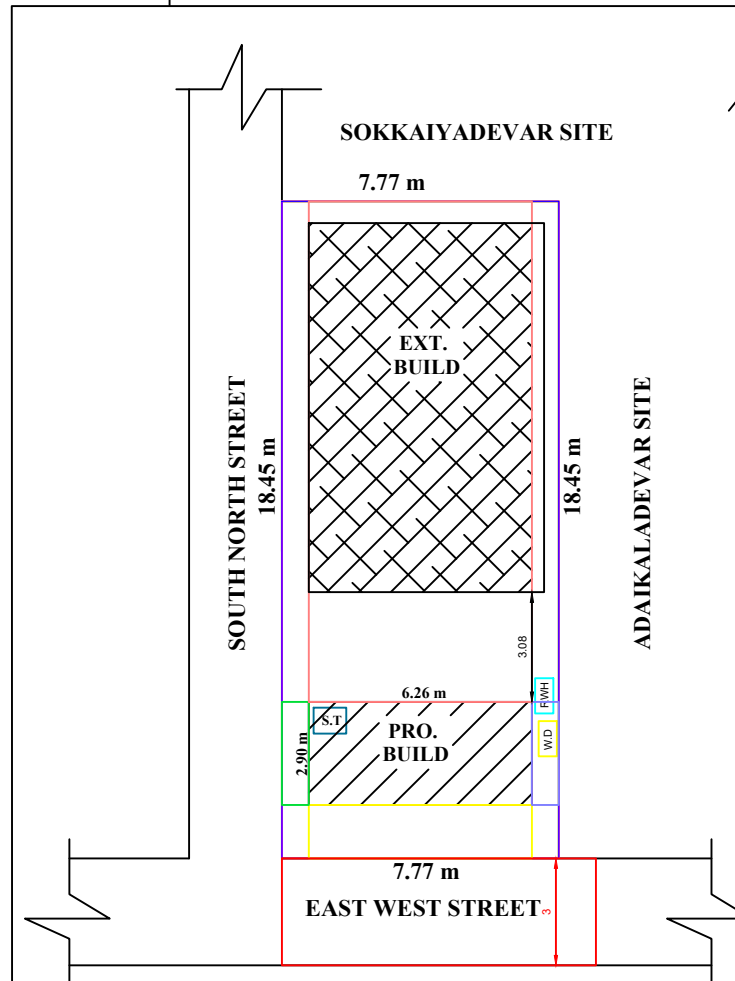
SITE PLAN
