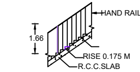
STAIRCASE
