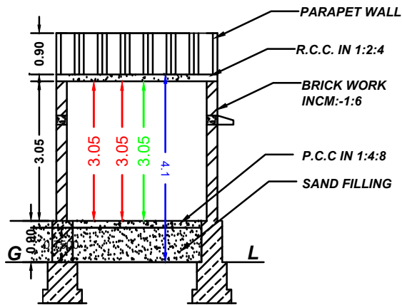
SECTION "AB"
