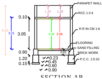
SECTION AB
