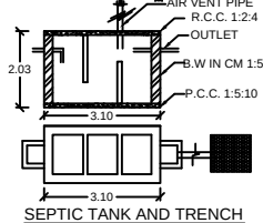
SEPTIC TANK AND TRENCH
