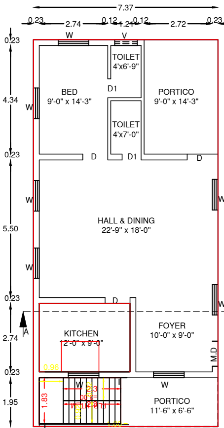
G.F. PLAN
