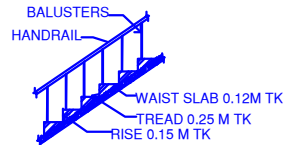
STAIRCASE DETAILS
