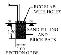
SECTION OF BS
