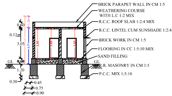
SECTION OF "BS"
