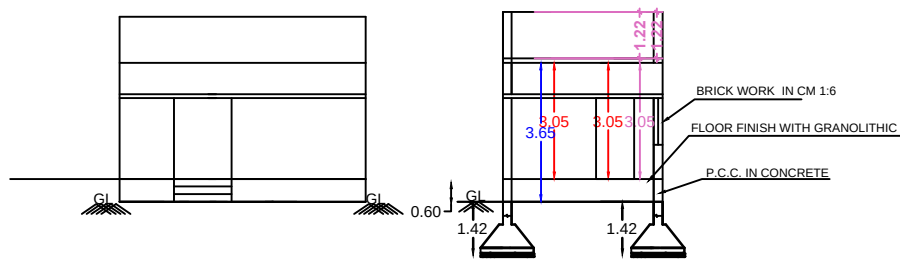
ELEVATION 6.48M SECTION ON AA
