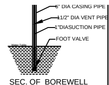
SEC. OF BOREWELL
