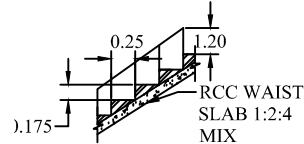
STAIR CASE DETAILS
