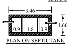
PLAN ON SEPTICTANK
