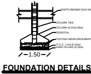
FOUNDATION DETAILS
