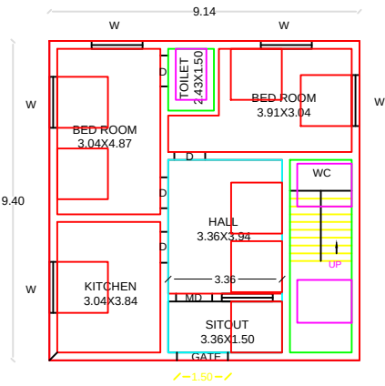
PROPOSED GF PLAN
