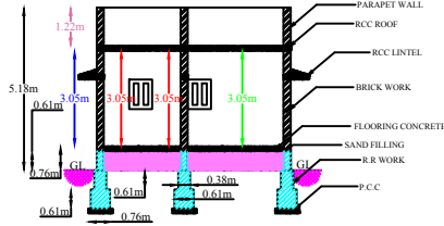
SECTION AB
