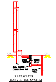
RAIN WATER HARVESTING SYSTEM
