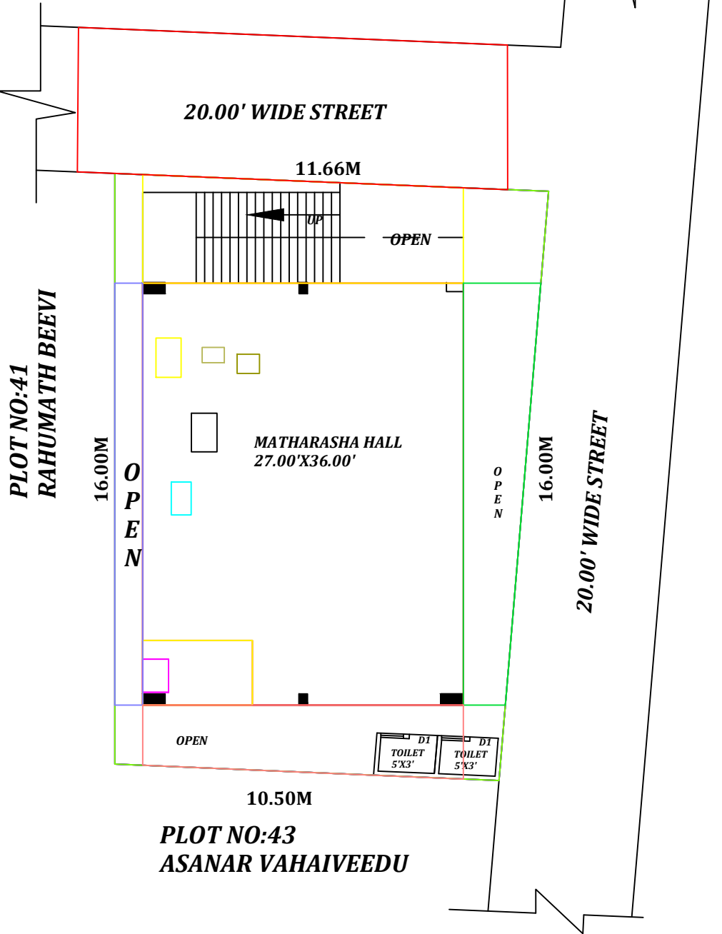
SITE PLAN
