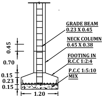
COLUMN DETAILS SCALE - 1:50
