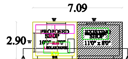
PRO.SHOP EX.SHOP GROUND FLOOR PLAN
