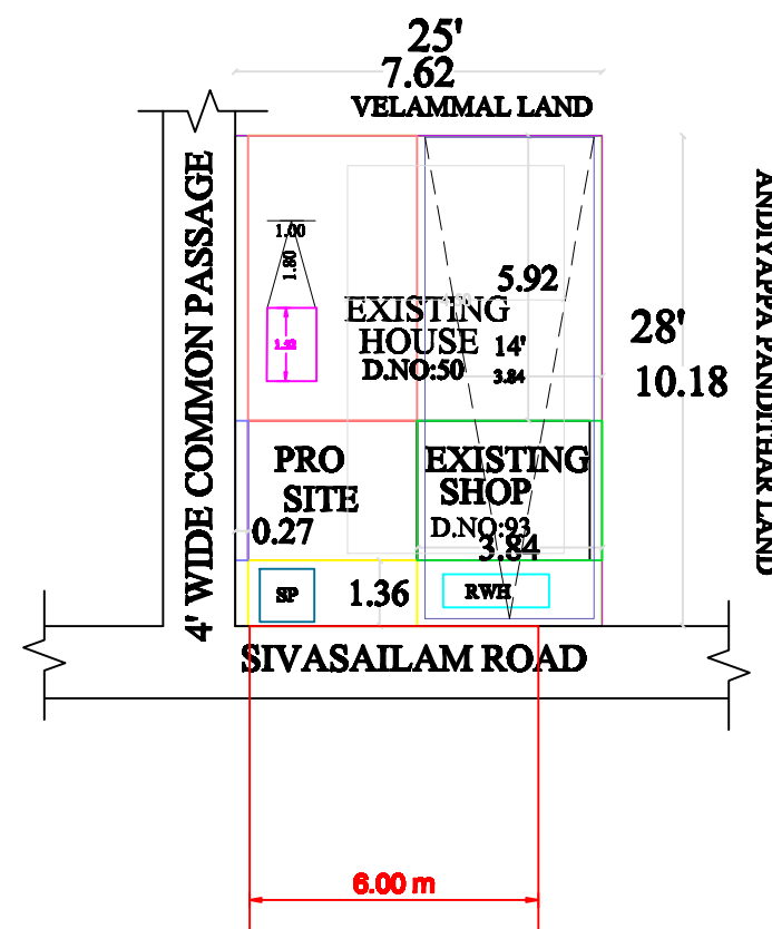
SITE PLAN
