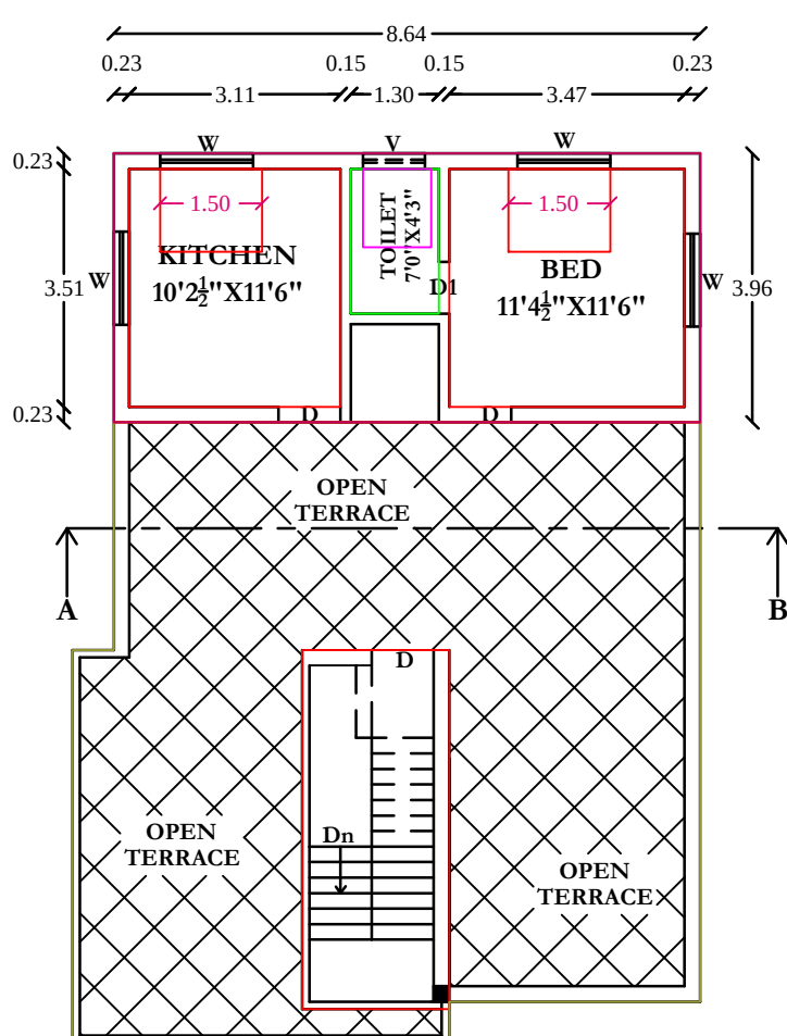
PRO.SECOND FLOOR PLAN
