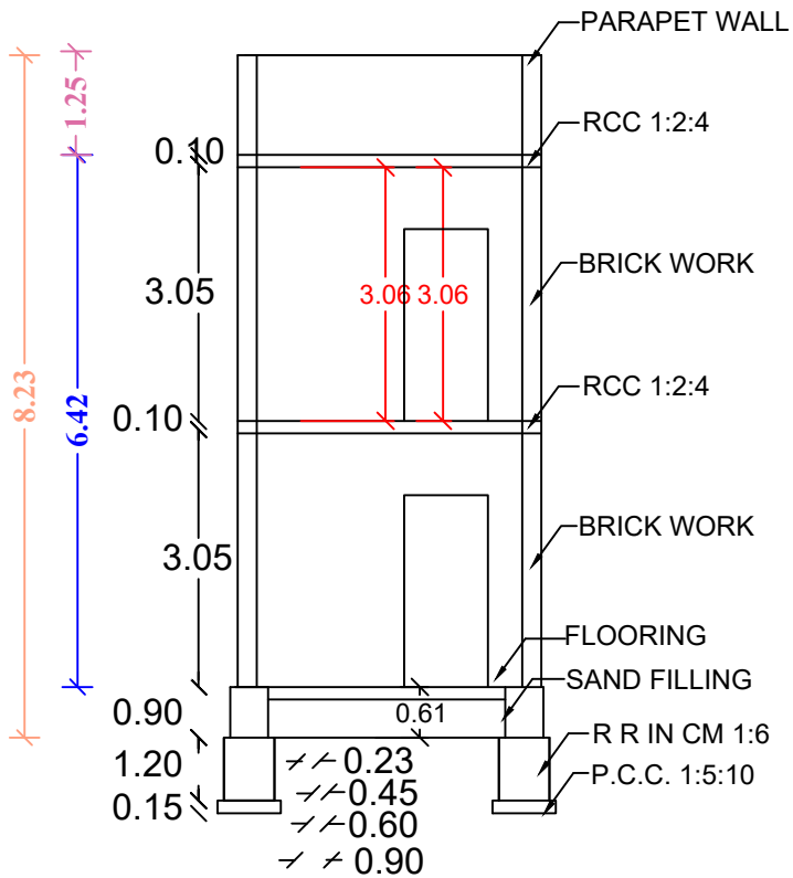
SECTION AB
