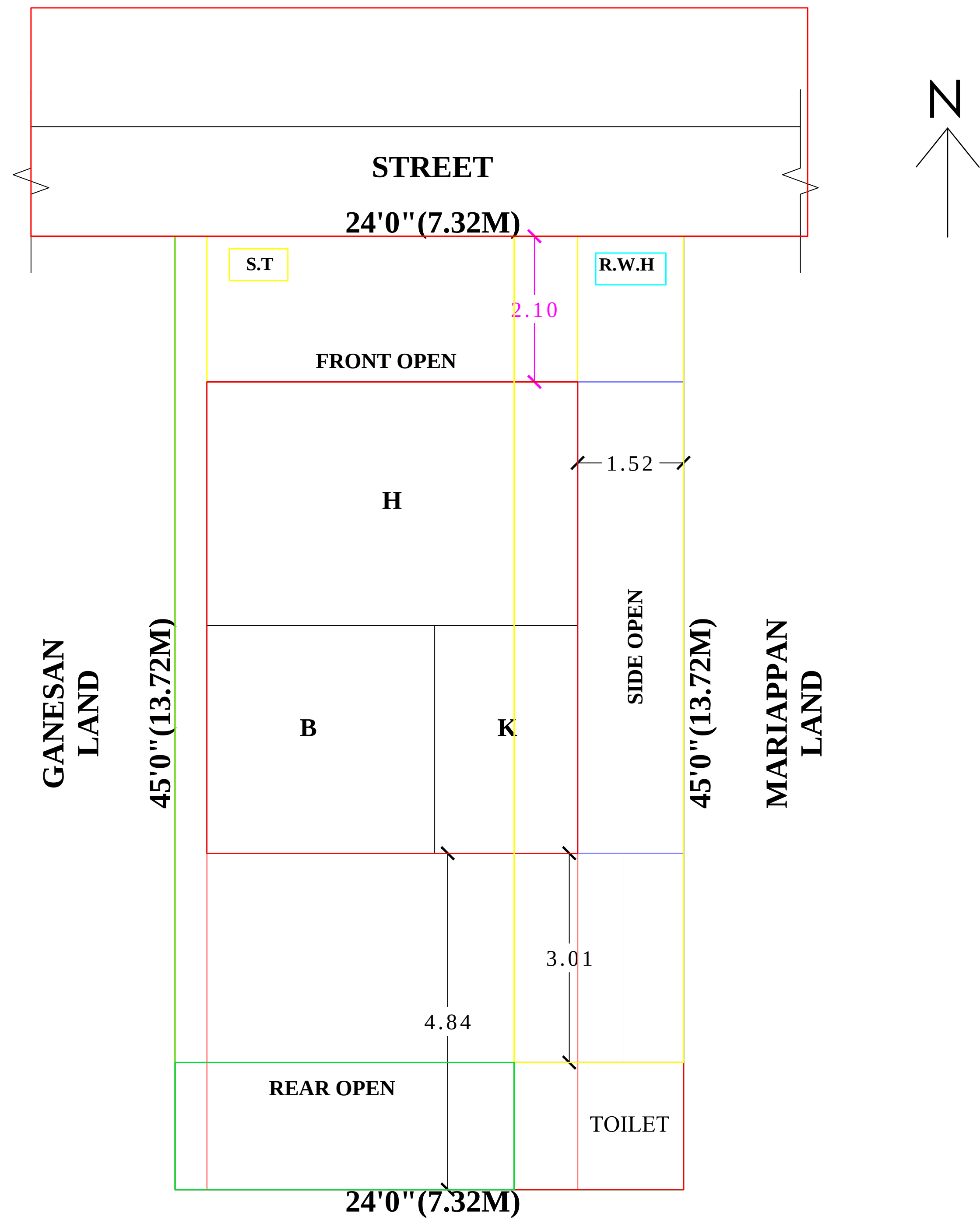
SITE PLAN
