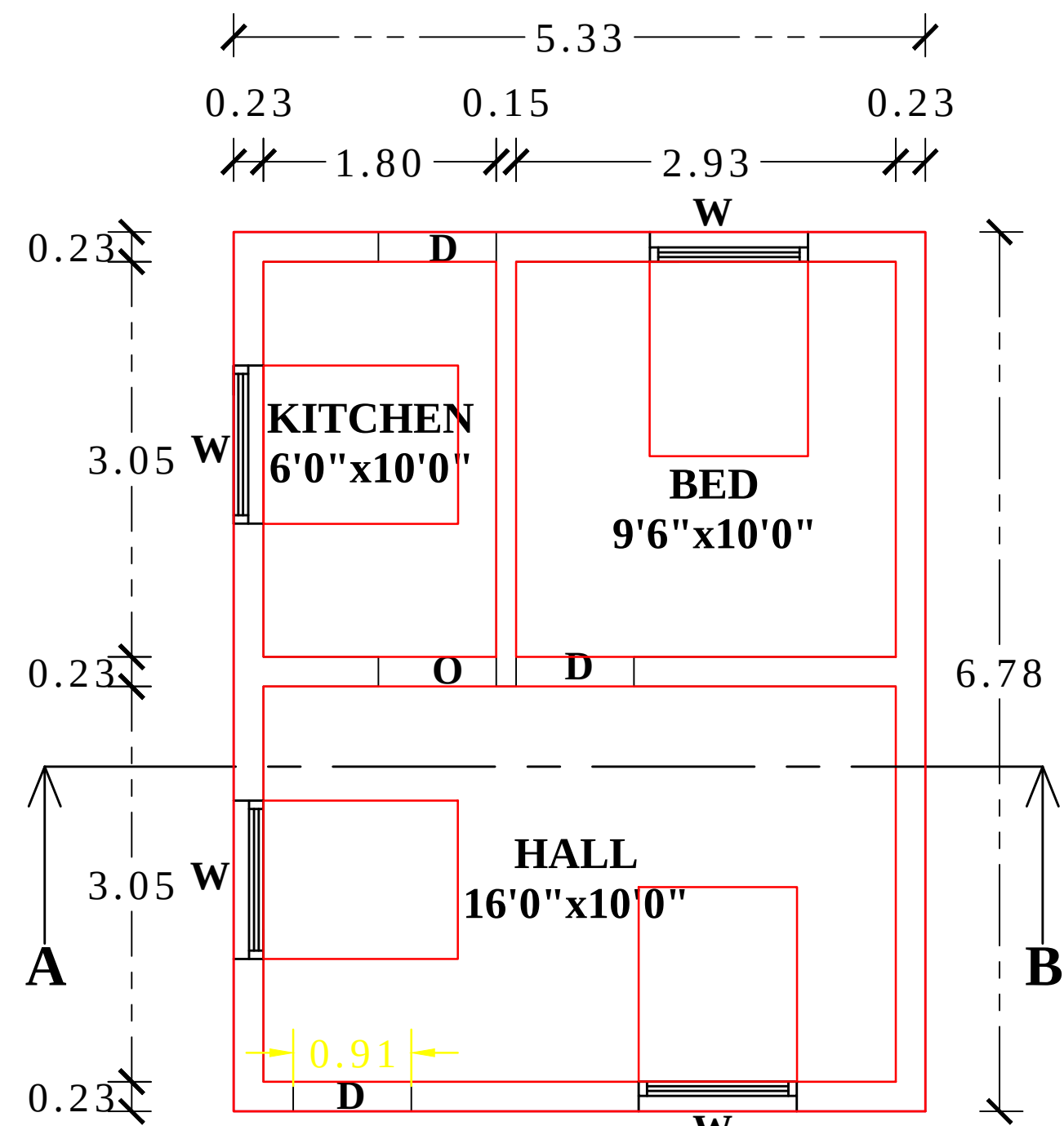
PLAN
