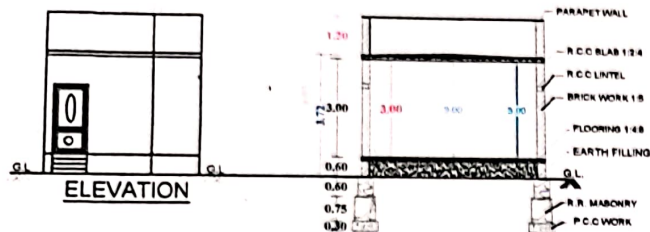
CROSS SECTION
