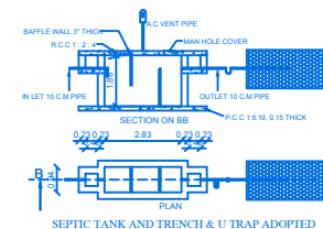
SEPTIC TANK AND TRENCH & U TRAP ADOPTED
