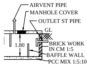
SECTION ON SEPTICTANK
