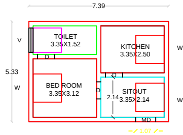
PROPOSED GF PLAN
