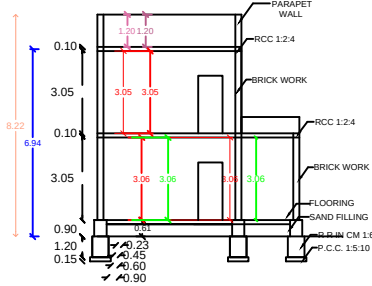
SECTION AB
