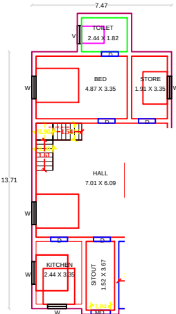
GROUND FLOC
