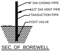
SEC. OF BOREWELL
