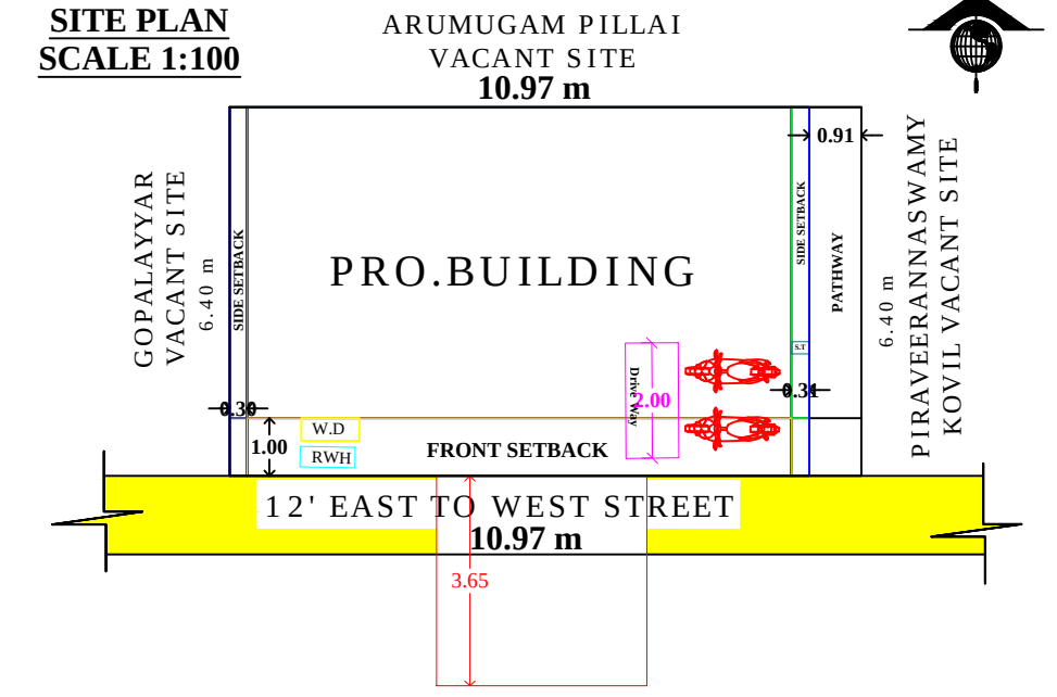
SITE PLAN
