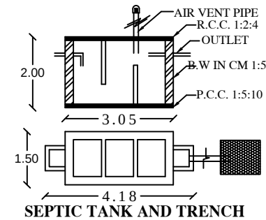
SEPTIC TANK AND TRENCH
