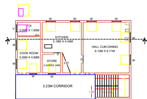
TYPICAL FLOOR PLAN-1 SLOPE=1IN12 PRO.GROUND FLOOR PLAN
