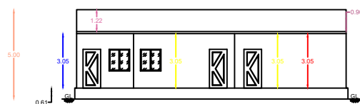
FRONT ELEVATION
