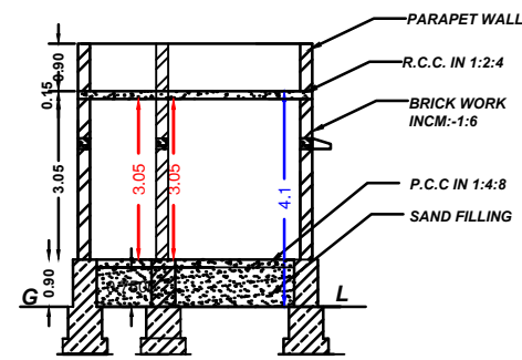
SECTION "AB"
