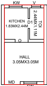
OUND FLOOR PLAN-2
