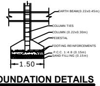
FOUNDATION DETAILS
