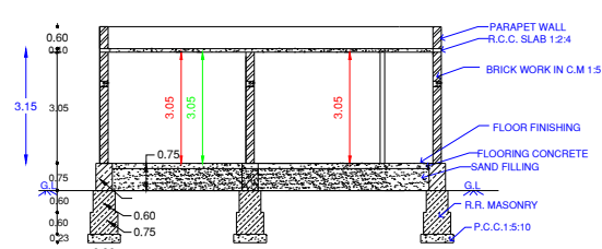
SECTION AB
