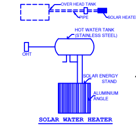
SOLAR WATER HEATER
