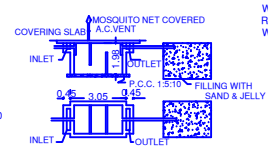
SEPTIC TANK & TRENCH U TRAP PROVISION
