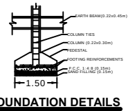
FOUNDATION DETAILS
