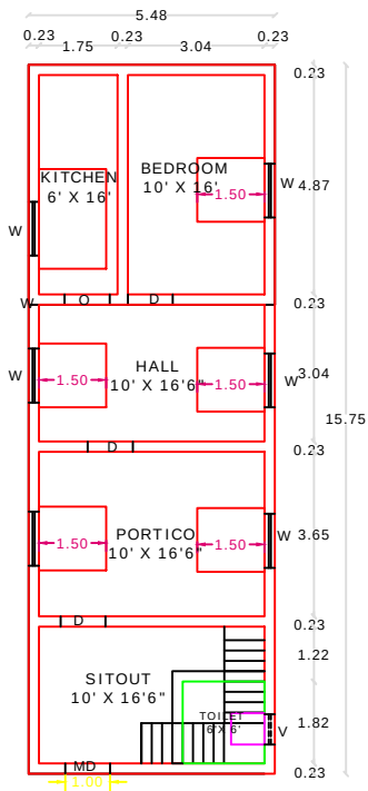
EXISTING GROUND FLOOR PLAN
