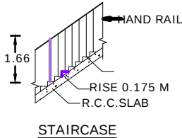
STAIRCASE
