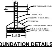
FOUNDATION DETAILS
