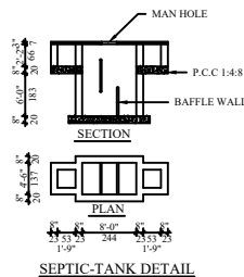
SEPTIC-TANK DETAIL
