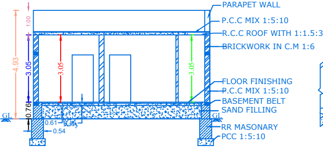
SECTION ON 'XX'
