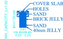
SECTION OF RAIN WATER COLLECTION TANK
