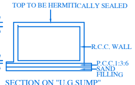
SECTION ON "U.G. SUMP"
