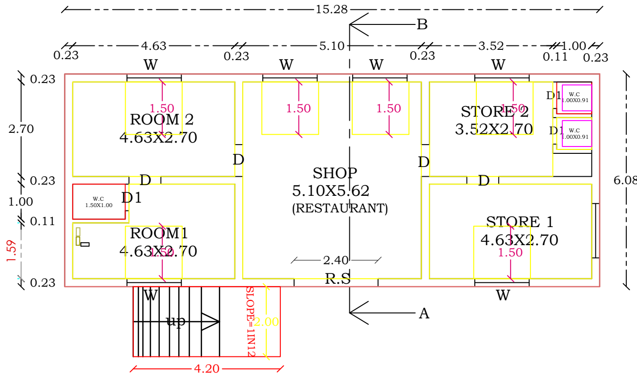
PLAN (BLOCK:3)
