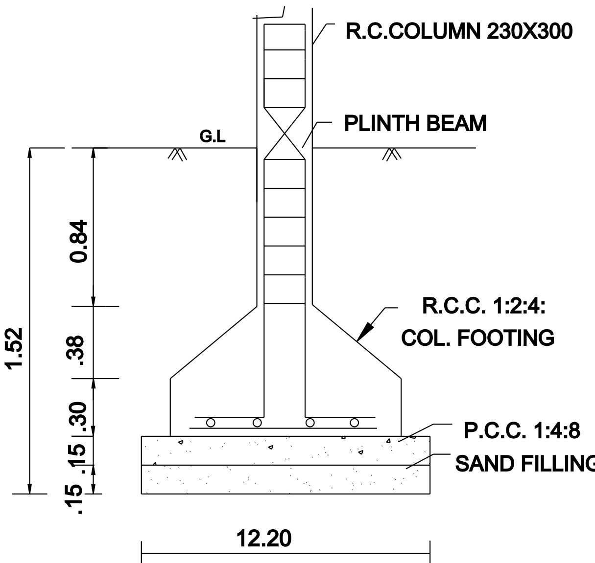
FOUNDATION DETAIL
