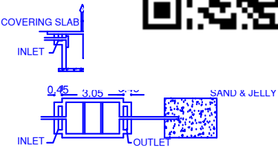
SEPTIC TANK & TRENCH U TRAP PROVISION
