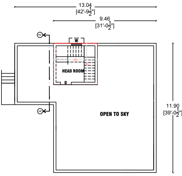
HEAD ROOM PLAN
