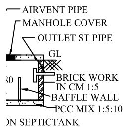
ON SEPTICTANK
