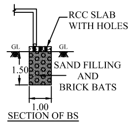
SECTION OF BS
