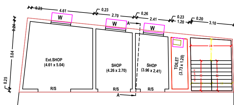
PLAN - GROUND FLOOR EXISTING - SHOP BUILDING
