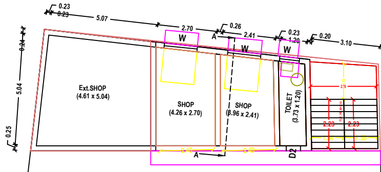
PLAN - FIRST FLOOR PROPOSED - SHOP BUILDING
