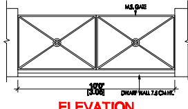
ELEVATION COMPOUND WALL DETAIL SCALE = 1 : 50
