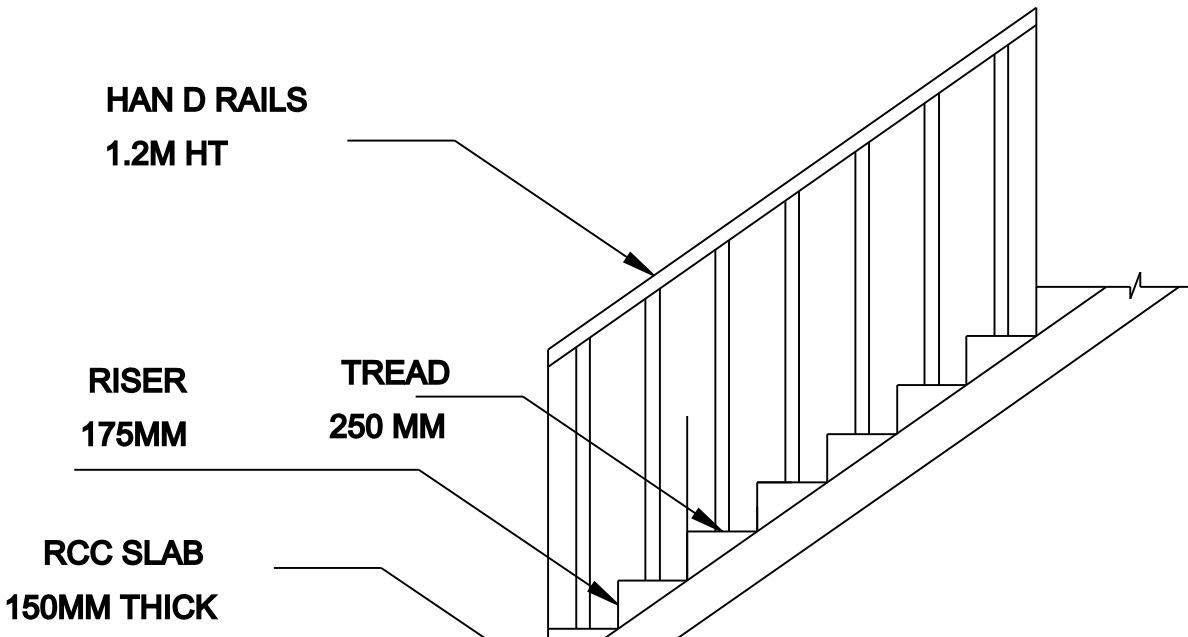
STAIRCASE DETAILS
