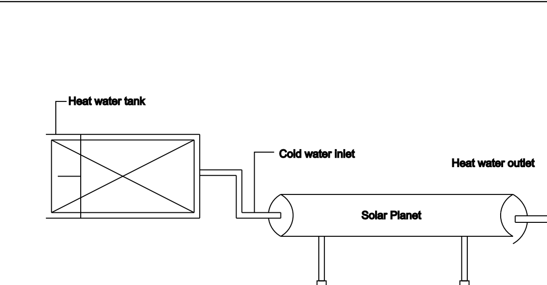
SOLAR WATER HEATER
