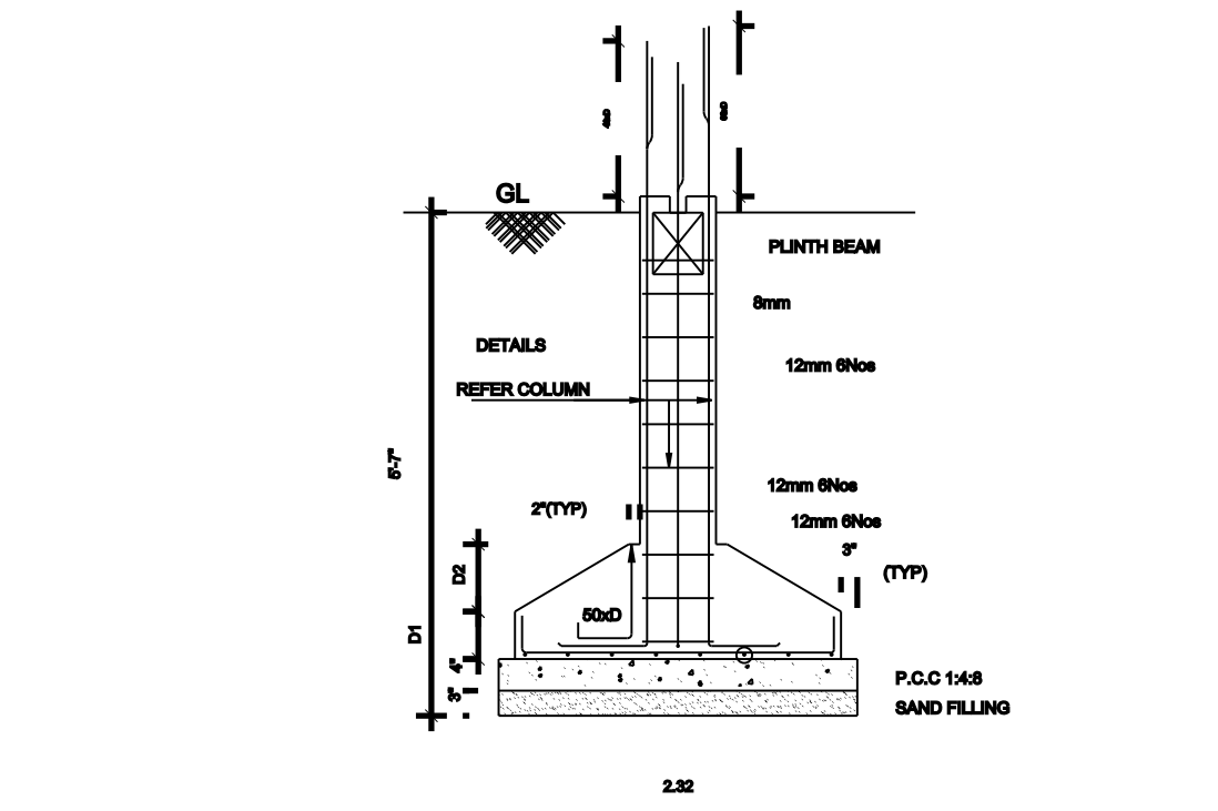
FOUNDATION DETAILS
